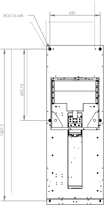
Rear View
